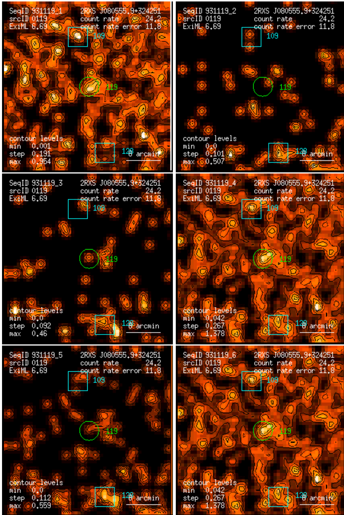
Figure 119: RASS 931119: detection 0119: band rate images, Gaussian filter: (1) PSPC channels 11 – 41, (2) 52 – 90, (3) 91 – 201, (4) 11 – 235, (5) 52 – 201, (6) 11 – 201. Broad band rates in counts/ks. Band rate contour levels in counts/ks/arcmin 2 .
