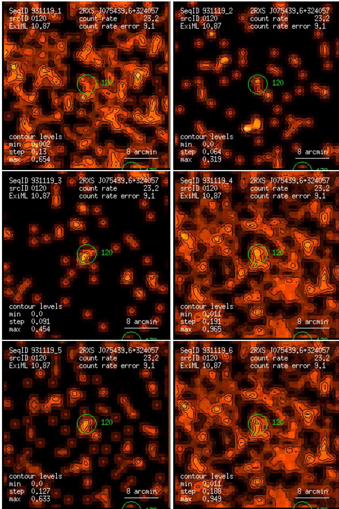
Figure 120: RASS 931119: detection 0120: band rate images, Gaussian filter: (1) PSPC channels 11 – 41, (2) 52 – 90, (3) 91 – 201, (4) 11 – 235, (5) 52 – 201, (6) 11 – 201. Broad band rates in counts/ks. Band rate contour levels in counts/ks/arcmin 2 .
