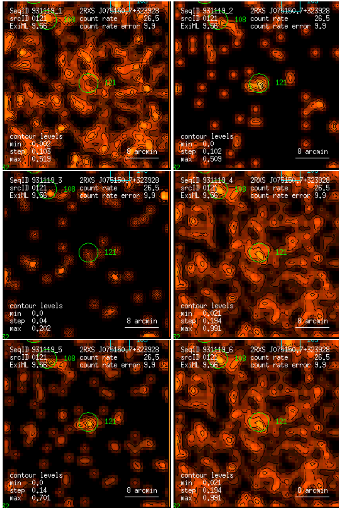
Figure 121: RASS 931119: detection 0121: band rate images, Gaussian filter: (1) PSPC channels 11 – 41, (2) 52 – 90, (3) 91 – 201, (4) 11 – 235, (5) 52 – 201, (6) 11 – 201. Broad band rates in counts/ks. Band rate contour levels in counts/ks/arcmin 2 .
