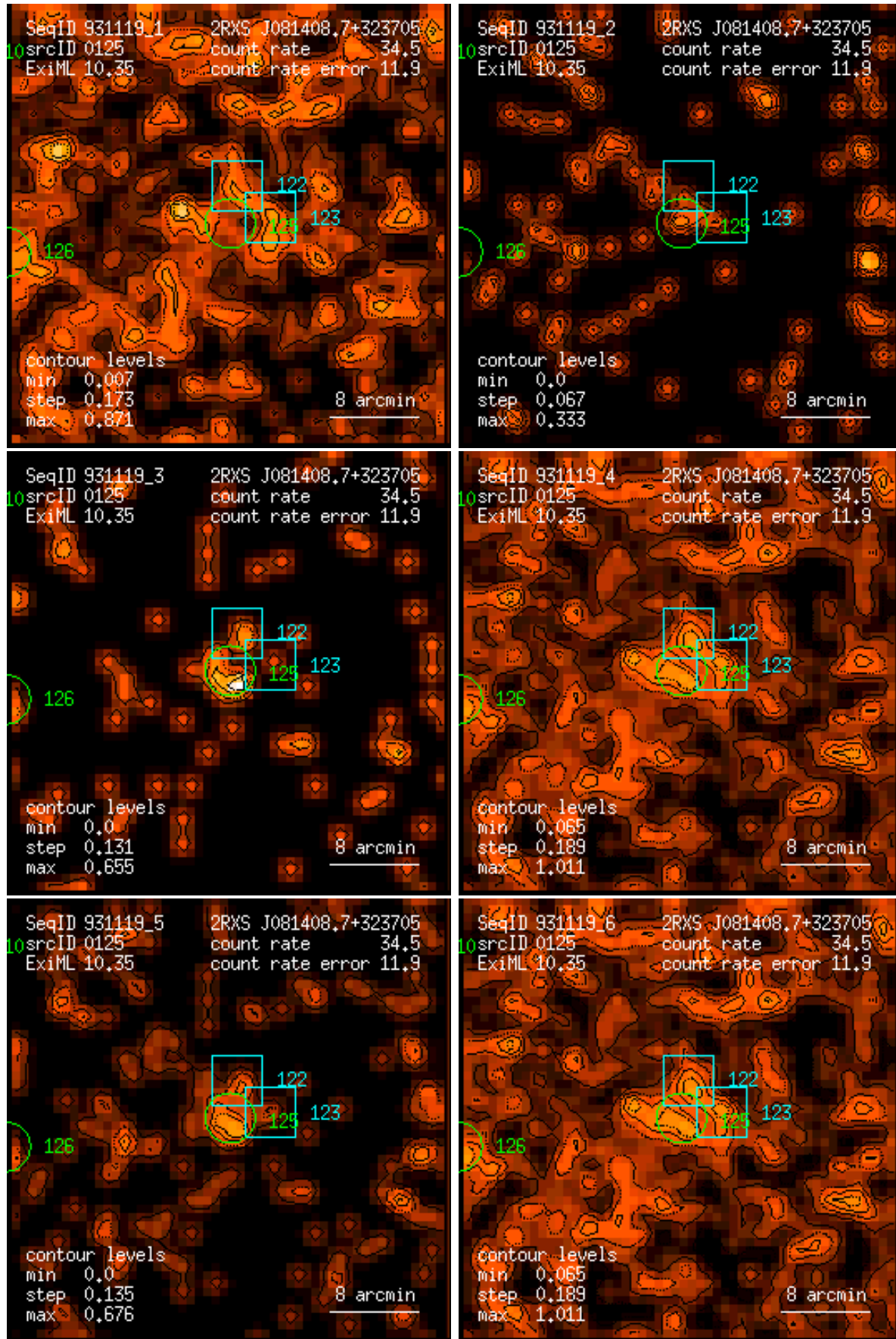
Figure 125: RASS 931119: detection 0125: band rate images, Gaussian filter: (1) PSPC channels 11 – 41, (2) 52 – 90, (3) 91 – 201, (4) 11 – 235, (5) 52 – 201, (6) 11 – 201. Broad band rates in counts/ks. Band rate contour levels in counts/ks/arcmin 2 .
