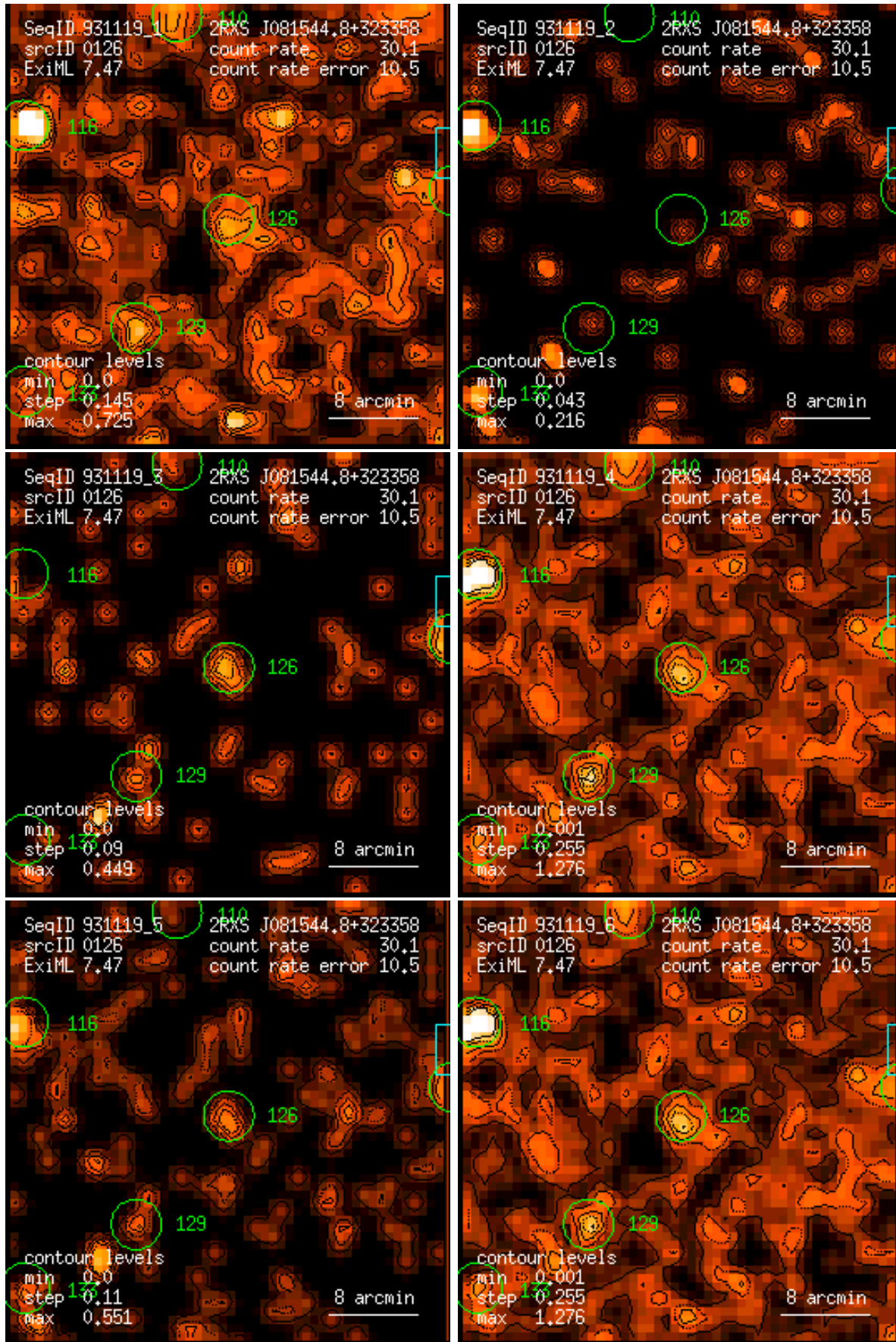
Figure 126: RASS 931119: detection 0126: band rate images, Gaussian filter: (1) PSPC channels 11 – 41, (2) 52 – 90, (3) 91 – 201, (4) 11 – 235, (5) 52 – 201, (6) 11 – 201. Broad band rates in counts/ks. Band rate contour levels in counts/ks/arcmin 2 .
