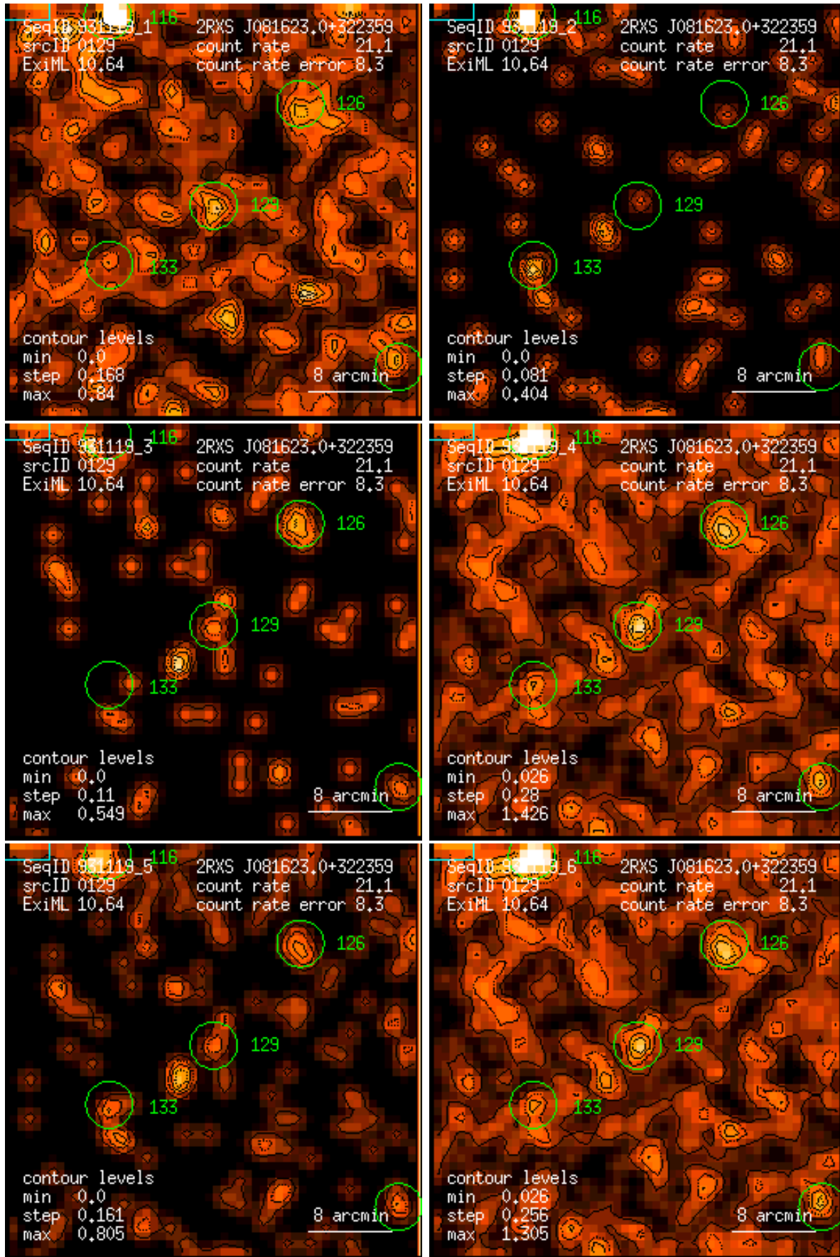
Figure 129: RASS 931119: detection 0129: band rate images, Gaussian filter: (1) PSPC channels 11 – 41, (2) 52 – 90, (3) 91 – 201, (4) 11 – 235, (5) 52 – 201, (6) 11 – 201. Broad band rates in counts/ks. Band rate contour levels in counts/ks/arcmin 2 .
