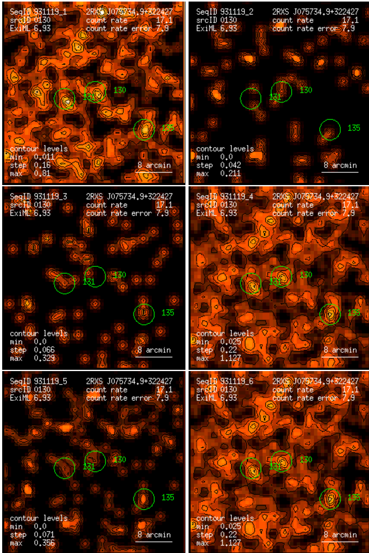
Figure 130: RASS 931119: detection 0130: band rate images, Gaussian filter: (1) PSPC channels 11 – 41, (2) 52 – 90, (3) 91 – 201, (4) 11 – 235, (5) 52 – 201, (6) 11 – 201. Broad band rates in counts/ks. Band rate contour levels in counts/ks/arcmin 2 .
