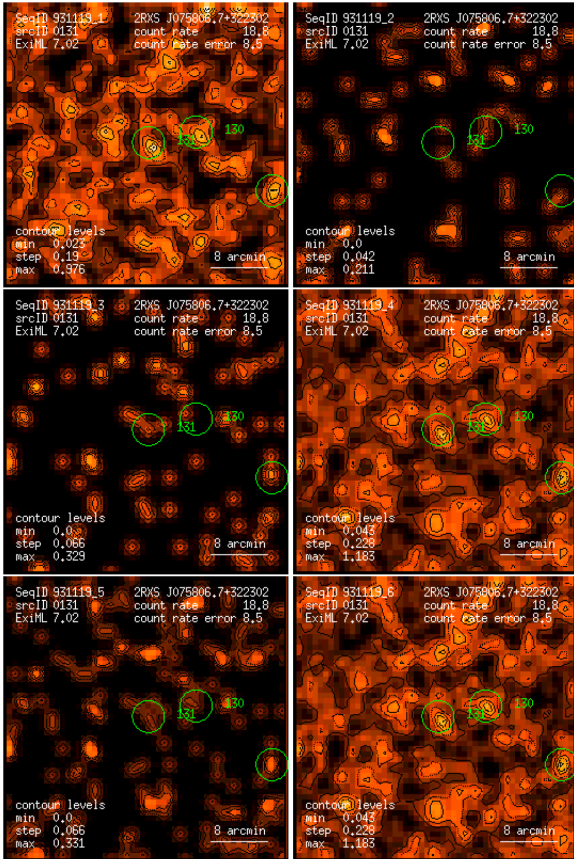
Figure 131: RASS 931119: detection 0131: band rate images, Gaussian filter: (1) PSPC channels 11 – 41, (2) 52 – 90, (3) 91 – 201, (4) 11 – 235, (5) 52 – 201, (6) 11 – 201. Broad band rates in counts/ks. Band rate contour levels in counts/ks/arcmin 2 .
