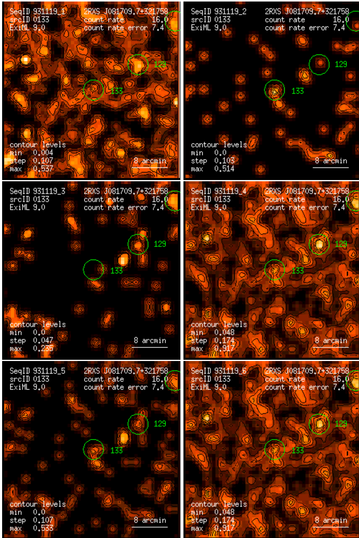
Figure 133: RASS 931119: detection 0133: band rate images, Gaussian filter: (1) PSPC channels 11 – 41, (2) 52 – 90, (3) 91 – 201, (4) 11 – 235, (5) 52 – 201, (6) 11 – 201. Broad band rates in counts/ks. Band rate contour levels in counts/ks/arcmin 2 .
