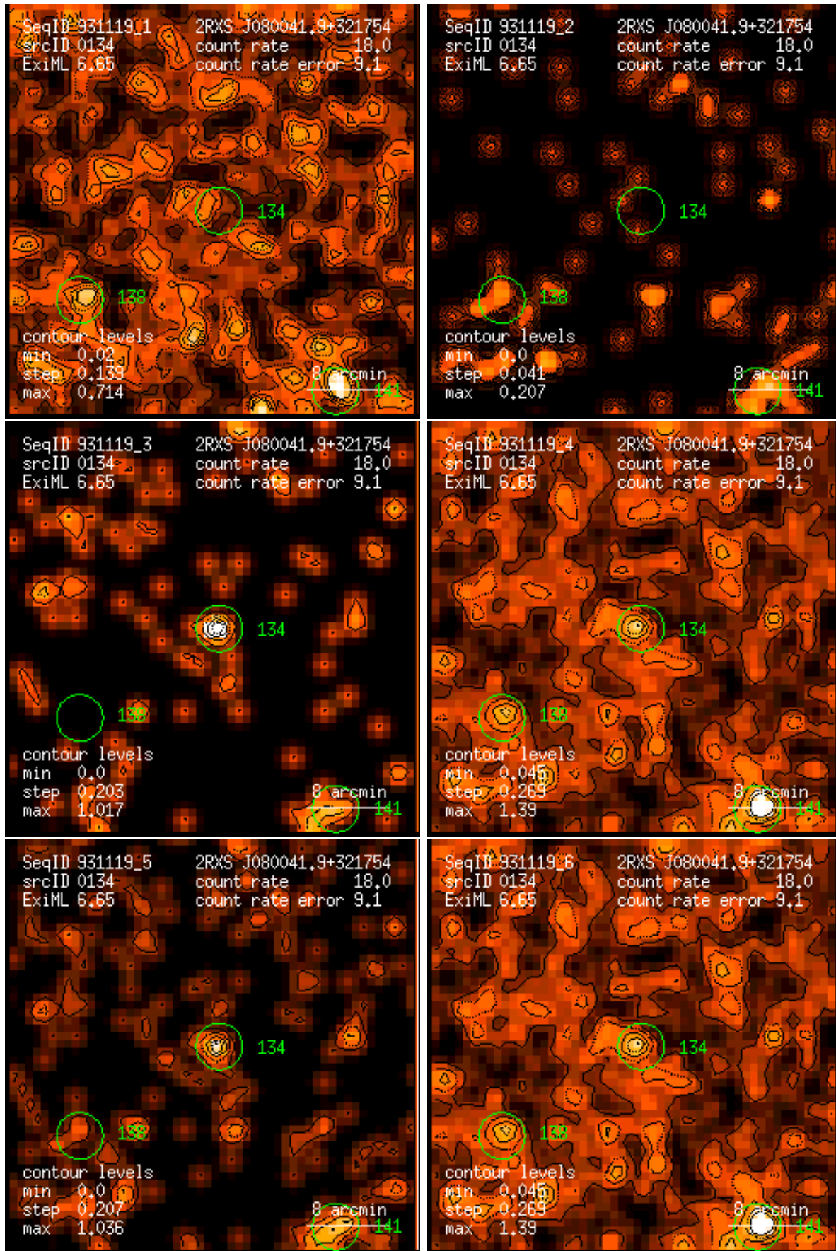
Figure 134: RASS 931119: detection 0134: band rate images, Gaussian filter: (1) PSPC channels 11 – 41, (2) 52 – 90, (3) 91 – 201, (4) 11 – 235, (5) 52 – 201, (6) 11 – 201. Broad band rates in counts/ks. Band rate contour levels in counts/ks/arcmin 2 .
