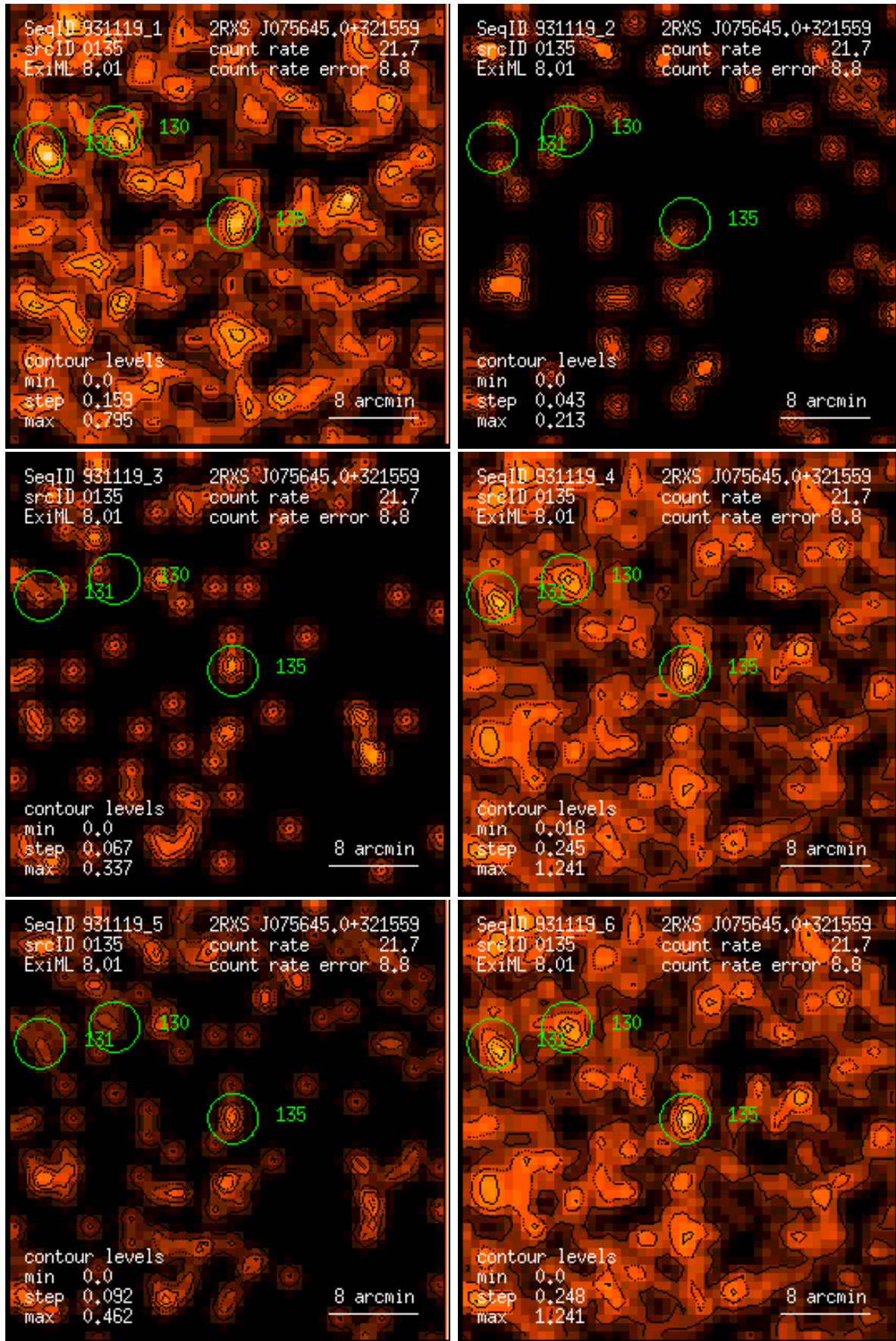
Figure 135: RASS 931119: detection 0135: band rate images, Gaussian filter: (1) PSPC channels 11 – 41, (2) 52 – 90, (3) 91 – 201, (4) 11 – 235, (5) 52 – 201, (6) 11 – 201. Broad band rates in counts/ks. Band rate contour levels in counts/ks/arcmin 2 .
