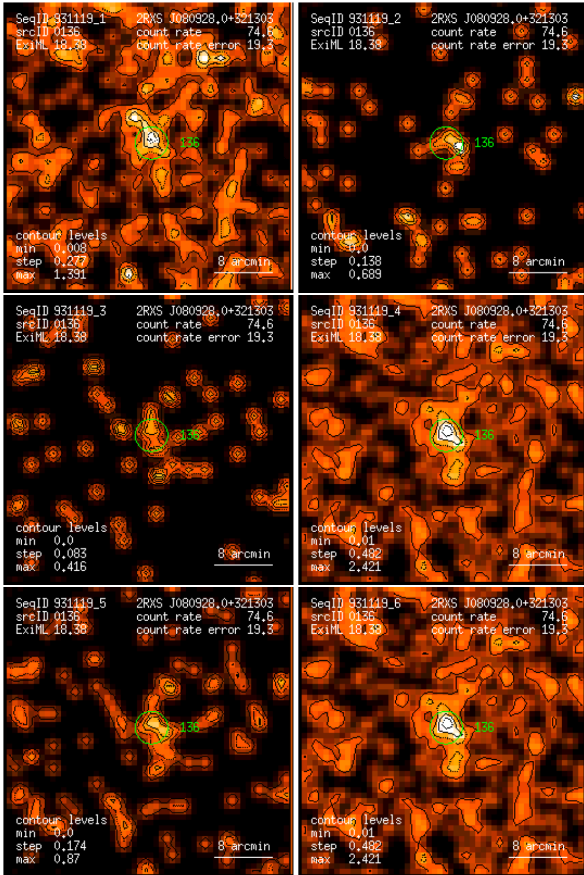
Figure 136: RASS 931119: detection 0136: band rate images, Gaussian filter: (1) PSPC channels 11 – 41, (2) 52 – 90, (3) 91 – 201, (4) 11 – 235, (5) 52 – 201, (6) 11 – 201. Broad band rates in counts/ks. Band rate contour levels in counts/ks/arcmin 2 .
