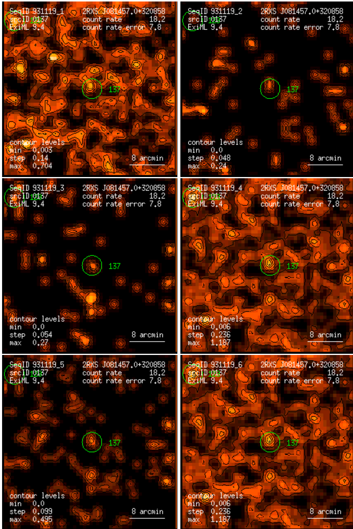
Figure 137: RASS 931119: detection 0137: band rate images, Gaussian filter: (1) PSPC channels 11 – 41, (2) 52 – 90, (3) 91 – 201, (4) 11 – 235, (5) 52 – 201, (6) 11 – 201. Broad band rates in counts/ks. Band rate contour levels in counts/ks/arcmin 2 .
