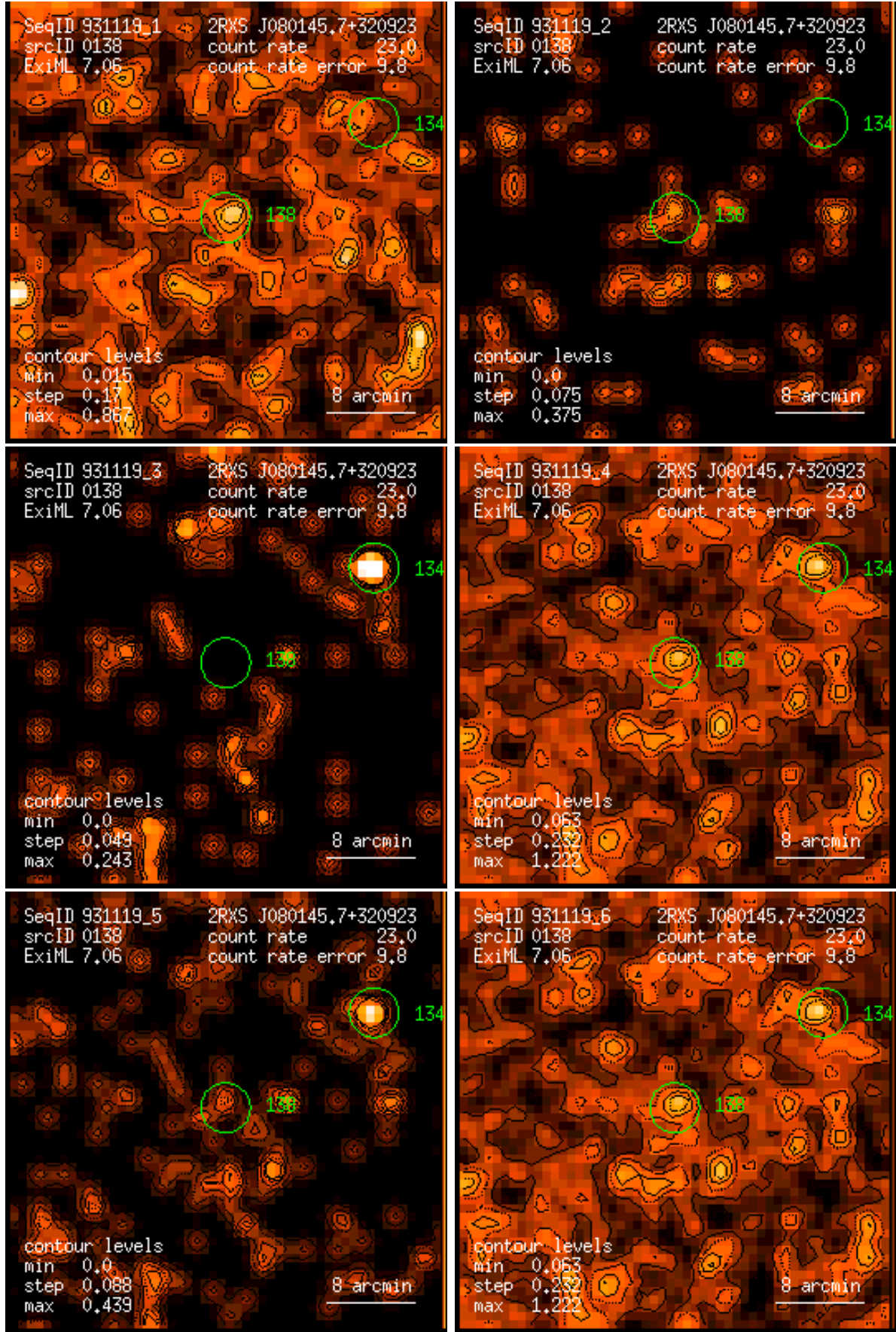
Figure 138: RASS 931119: detection 0138: band rate images, Gaussian filter: (1) PSPC channels 11 – 41, (2) 52 – 90, (3) 91 – 201, (4) 11 – 235, (5) 52 – 201, (6) 11 – 201. Broad band rates in counts/ks. Band rate contour levels in counts/ks/arcmin 2 .
