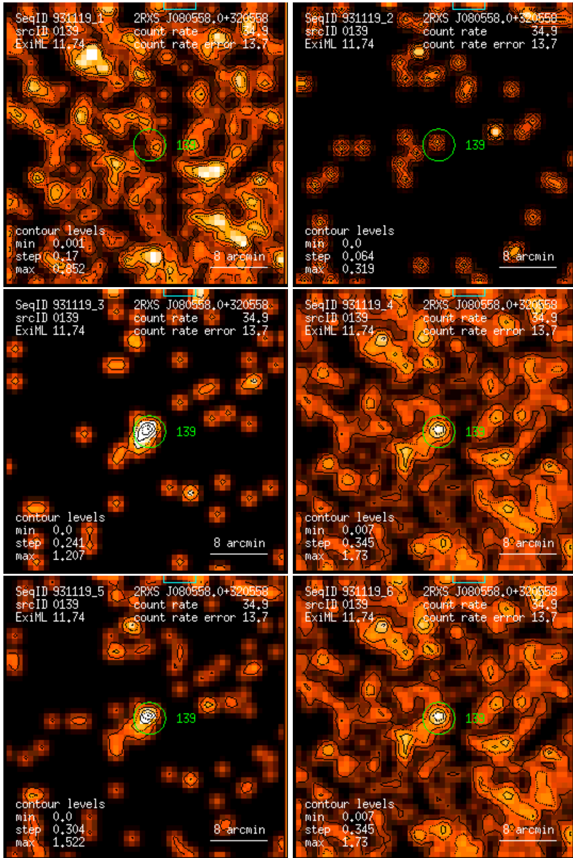
Figure 139: RASS 931119: detection 0139: band rate images, Gaussian filter: (1) PSPC channels 11 – 41, (2) 52 – 90, (3) 91 – 201, (4) 11 – 235, (5) 52 – 201, (6) 11 – 201. Broad band rates in counts/ks. Band rate contour levels in counts/ks/arcmin 2 .
