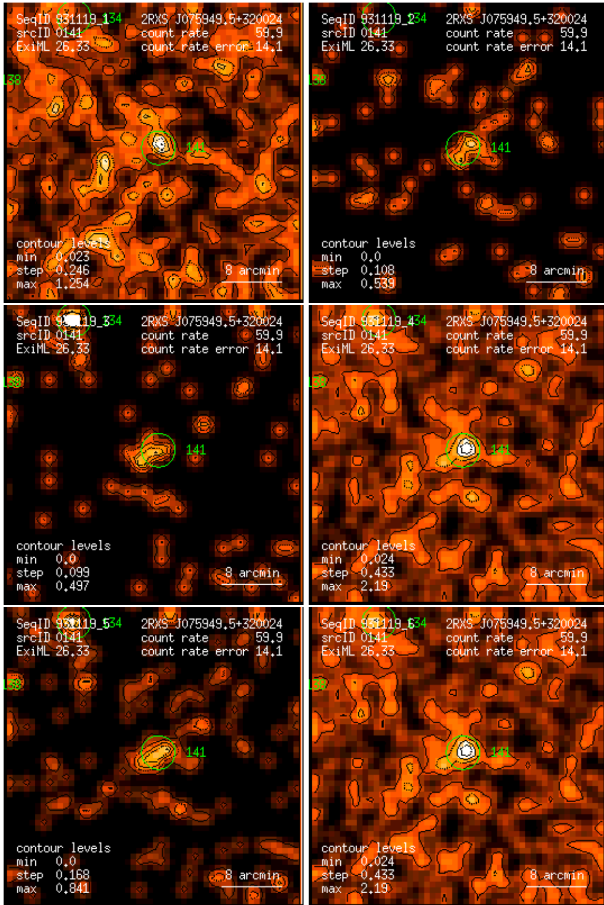
Figure 141: RASS 931119: detection 0141: band rate images, Gaussian filter: (1) PSPC channels 11 – 41, (2) 52 – 90, (3) 91 – 201, (4) 11 – 235, (5) 52 – 201, (6) 11 – 201. Broad band rates in counts/ks. Band rate contour levels in counts/ks/arcmin 2 .
