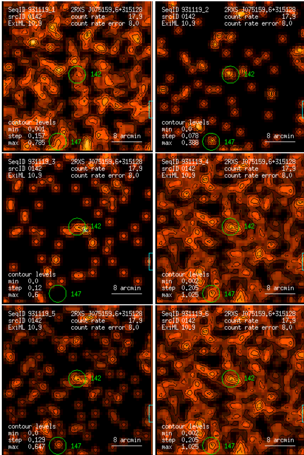
Figure 142: RASS 931119: detection 0142: band rate images, Gaussian filter: (1) PSPC channels 11 – 41, (2) 52 – 90, (3) 91 – 201, (4) 11 – 235, (5) 52 – 201, (6) 11 – 201. Broad band rates in counts/ks. Band rate contour levels in counts/ks/arcmin 2 .
