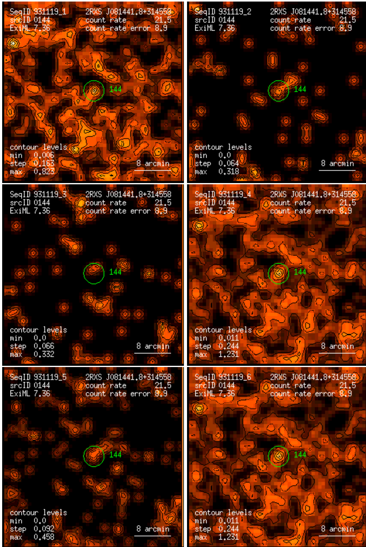
Figure 144: RASS 931119: detection 0144: band rate images, Gaussian filter: (1) PSPC channels 11 – 41, (2) 52 – 90, (3) 91 – 201, (4) 11 – 235, (5) 52 – 201, (6) 11 – 201. Broad band rates in counts/ks. Band rate contour levels in counts/ks/arcmin 2 .
