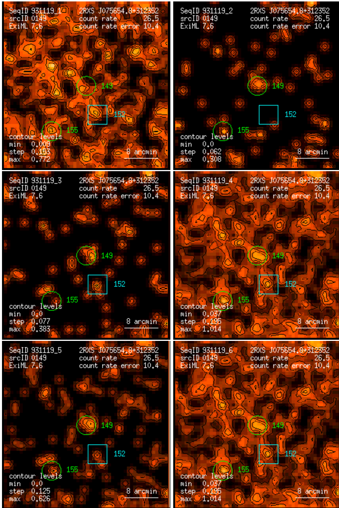
Figure 149: RASS 931119: detection 0149: band rate images, Gaussian filter: (1) PSPC channels 11 – 41, (2) 52 – 90, (3) 91 – 201, (4) 11 – 235, (5) 52 – 201, (6) 11 – 201. Broad band rates in counts/ks. Band rate contour levels in counts/ks/arcmin 2 .
