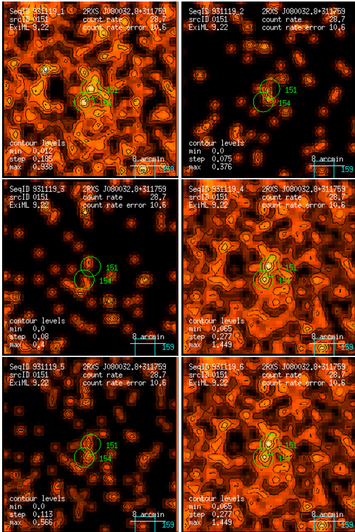
Figure 151: RASS 931119: detection 0151: band rate images, Gaussian filter: (1) PSPC channels 11 – 41, (2) 52 – 90, (3) 91 – 201, (4) 11 – 235, (5) 52 – 201, (6) 11 – 201. Broad band rates in counts/ks. Band rate contour levels in counts/ks/arcmin 2 .
