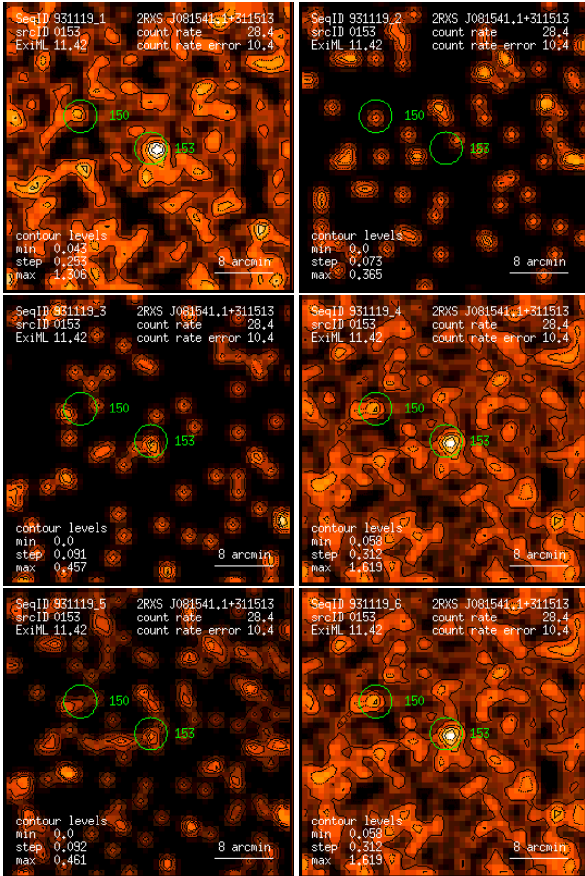
Figure 153: RASS 931119: detection 0153: band rate images, Gaussian filter: (1) PSPC channels 11 – 41, (2) 52 – 90, (3) 91 – 201, (4) 11 – 235, (5) 52 – 201, (6) 11 – 201. Broad band rates in counts/ks. Band rate contour levels in counts/ks/arcmin 2 .
