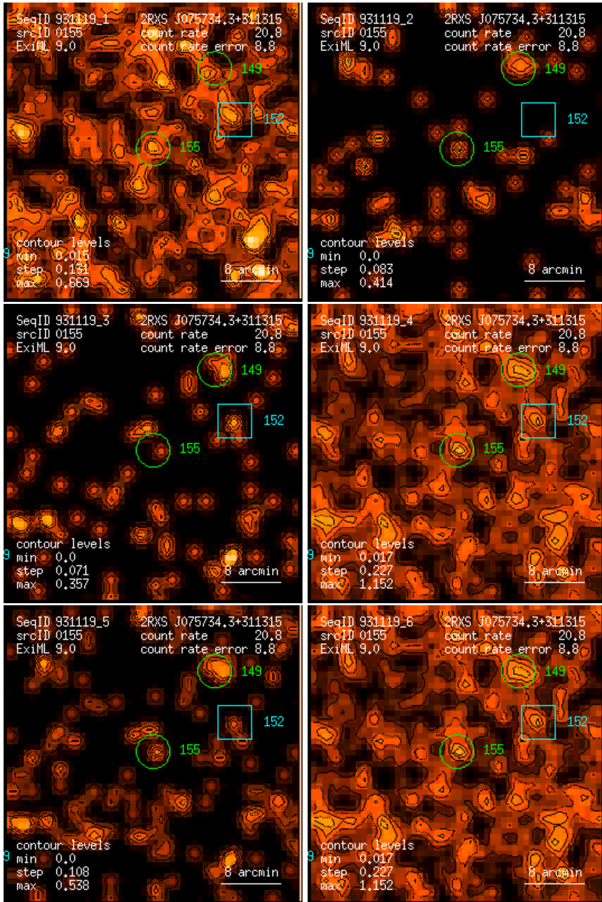
Figure 155: RASS 931119: detection 0155: band rate images, Gaussian filter: (1) PSPC channels 11 – 41, (2) 52 – 90, (3) 91 – 201, (4) 11 – 235, (5) 52 – 201, (6) 11 – 201. Broad band rates in counts/ks. Band rate contour levels in counts/ks/arcmin 2 .
