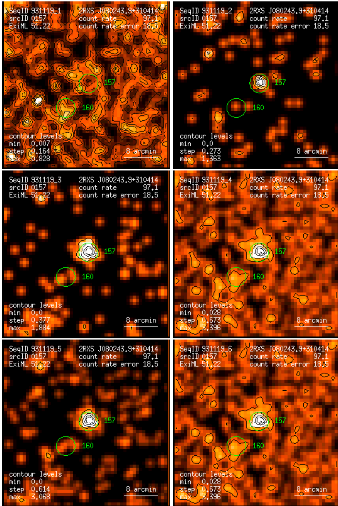
Figure 157: RASS 931119: detection 0157: band rate images, Gaussian filter: (1) PSPC channels 11 – 41, (2) 52 – 90, (3) 91 – 201, (4) 11 – 235, (5) 52 – 201, (6) 11 – 201. Broad band rates in counts/ks. Band rate contour levels in counts/ks/arcmin 2 .
