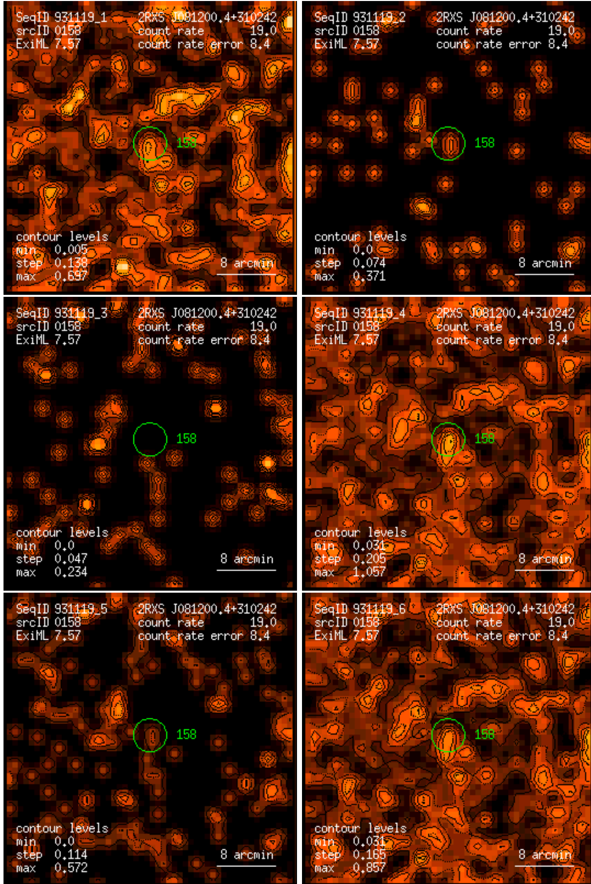
Figure 158: RASS 931119: detection 0158: band rate images, Gaussian filter: (1) PSPC channels 11 – 41, (2) 52 – 90, (3) 91 – 201, (4) 11 – 235, (5) 52 – 201, (6) 11 – 201. Broad band rates in counts/ks. Band rate contour levels in counts/ks/arcmin 2 .
