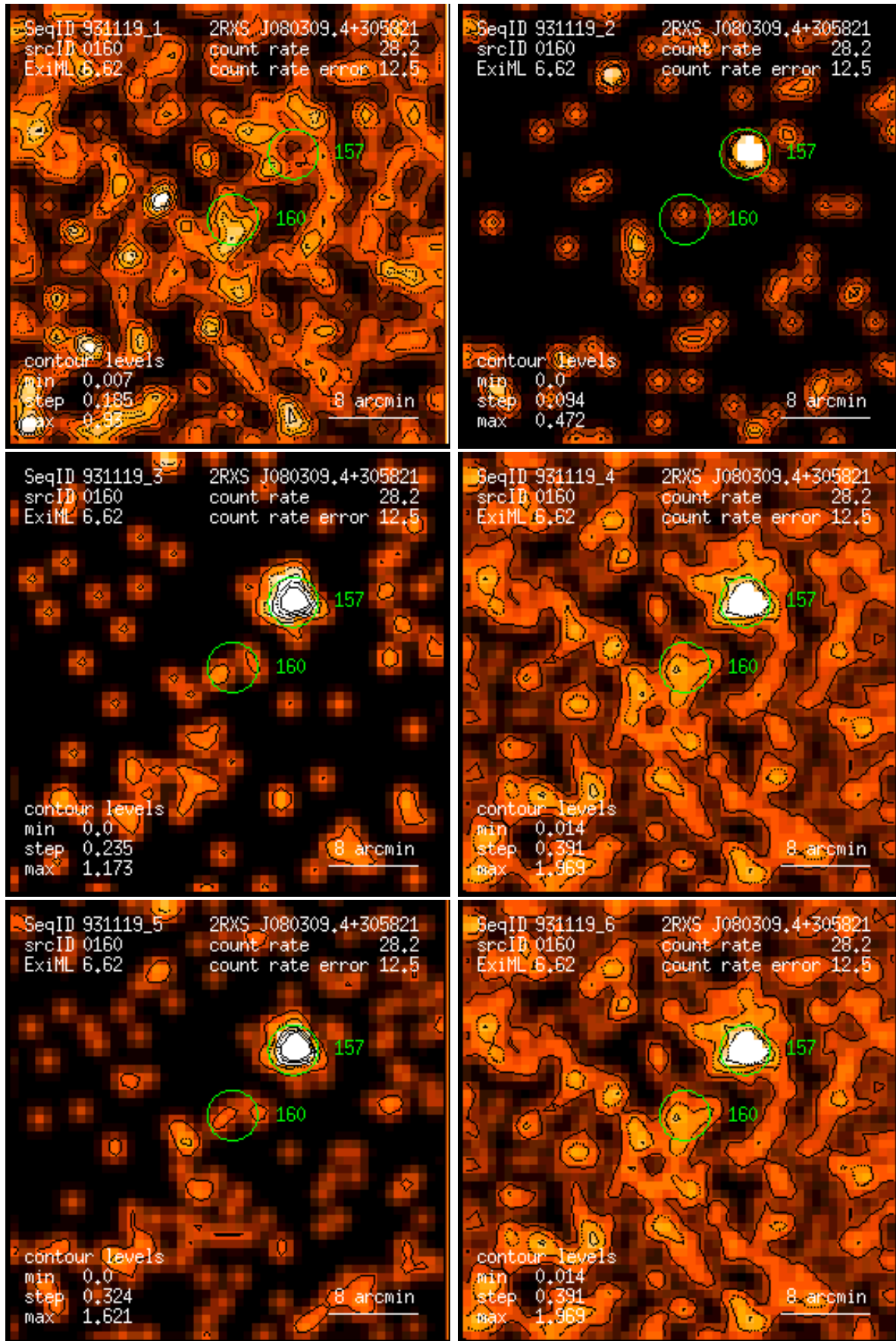
Figure 160: RASS 931119: detection 0160: band rate images, Gaussian filter: (1) PSPC channels 11 – 41, (2) 52 – 90, (3) 91 – 201, (4) 11 – 235, (5) 52 – 201, (6) 11 – 201. Broad band rates in counts/ks. Band rate contour levels in counts/ks/arcmin 2 .
