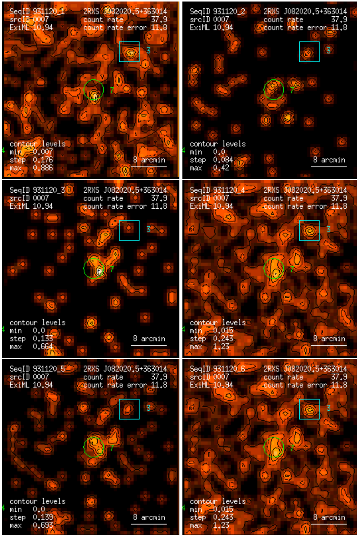
Figure 7: RASS 931120: detection 0007: band rate images, Gaussian filter: (1) PSPC channels 11 – 41, (2) 52 – 90, (3) 91 – 201, (4) 11 – 235, (5) 52 – 201, (6) 11 – 201. Broad band rates in counts/ks. Band rate contour levels in counts/ks/arcmin 2 .
