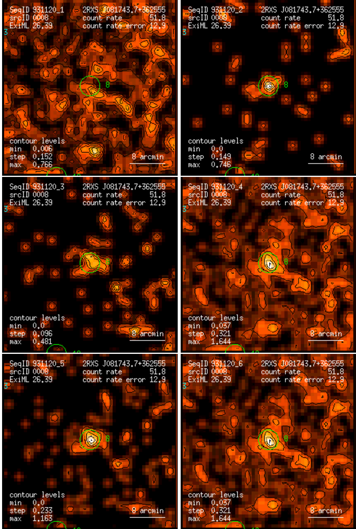
Figure 8: RASS 931120: detection 0008: band rate images, Gaussian filter: (1) PSPC channels 11 – 41, (2) 52 – 90, (3) 91 – 201, (4) 11 – 235, (5) 52 – 201, (6) 11 – 201. Broad band rates in counts/ks. Band rate contour levels in counts/ks/arcmin 2 .
