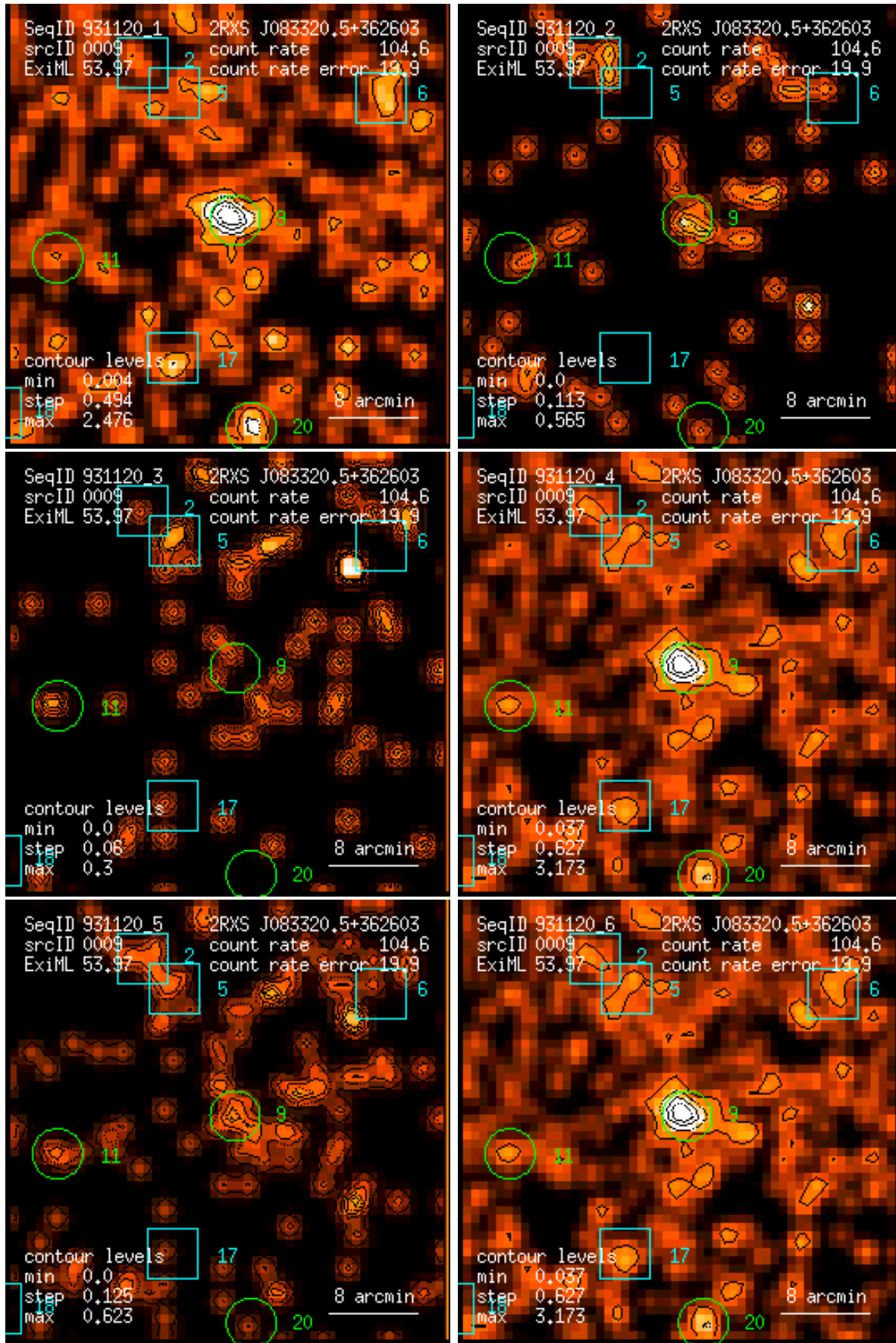
Figure 9: RASS 931120: detection 0009: band rate images, Gaussian filter: (1) PSPC channels 11 – 41, (2) 52 – 90, (3) 91 – 201, (4) 11 – 235, (5) 52 – 201, (6) 11 – 201. Broad band rates in counts/ks. Band rate contour levels in counts/ks/arcmin 2 .
