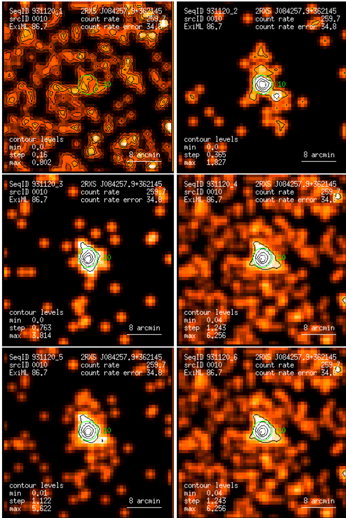
Figure 10: RASS 931120: detection 0010: band rate images, Gaussian filter: (1) PSPC channels 11 – 41, (2) 52 – 90, (3) 91 – 201, (4) 11 – 235, (5) 52 – 201, (6) 11 – 201. Broad band rates in counts/ks. Band rate contour levels in counts/ks/arcmin 2 .
