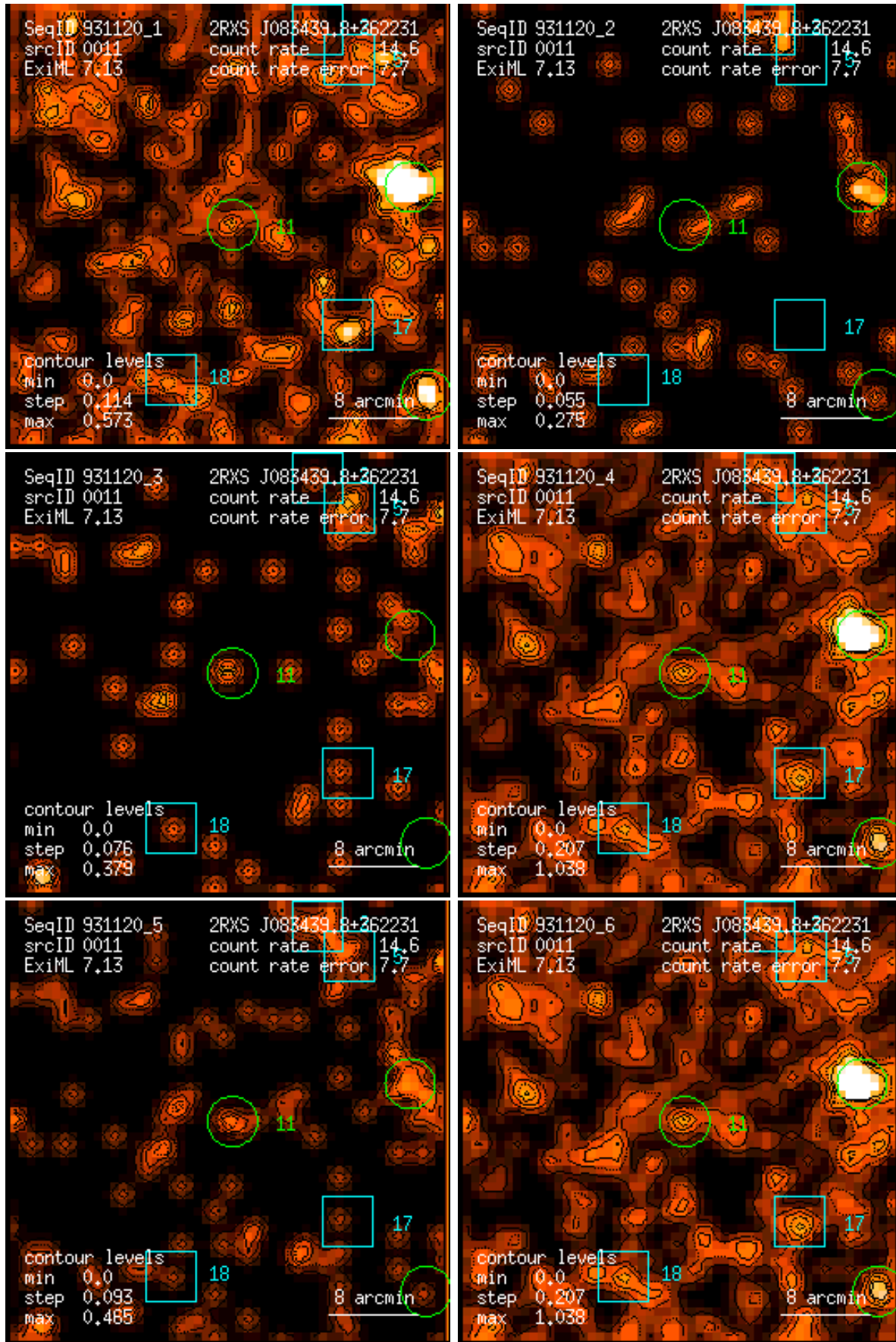
Figure 11: RASS 931120: detection 0011: band rate images, Gaussian filter: (1) PSPC channels 11 – 41, (2) 52 – 90, (3) 91 – 201, (4) 11 – 235, (5) 52 – 201, (6) 11 – 201. Broad band rates in counts/ks. Band rate contour levels in counts/ks/arcmin 2 .
