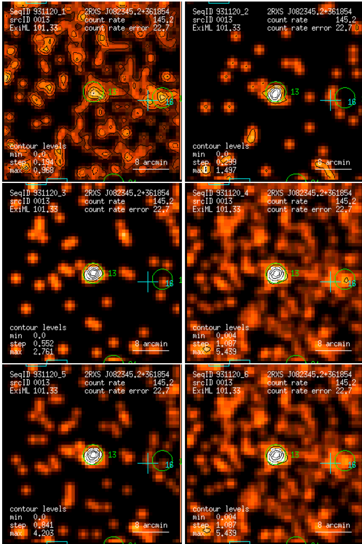
Figure 13: RASS 931120: detection 0013: band rate images, Gaussian filter: (1) PSPC channels 11 – 41, (2) 52 – 90, (3) 91 – 201, (4) 11 – 235, (5) 52 – 201, (6) 11 – 201. Broad band rates in counts/ks. Band rate contour levels in counts/ks/arcmin 2 .
