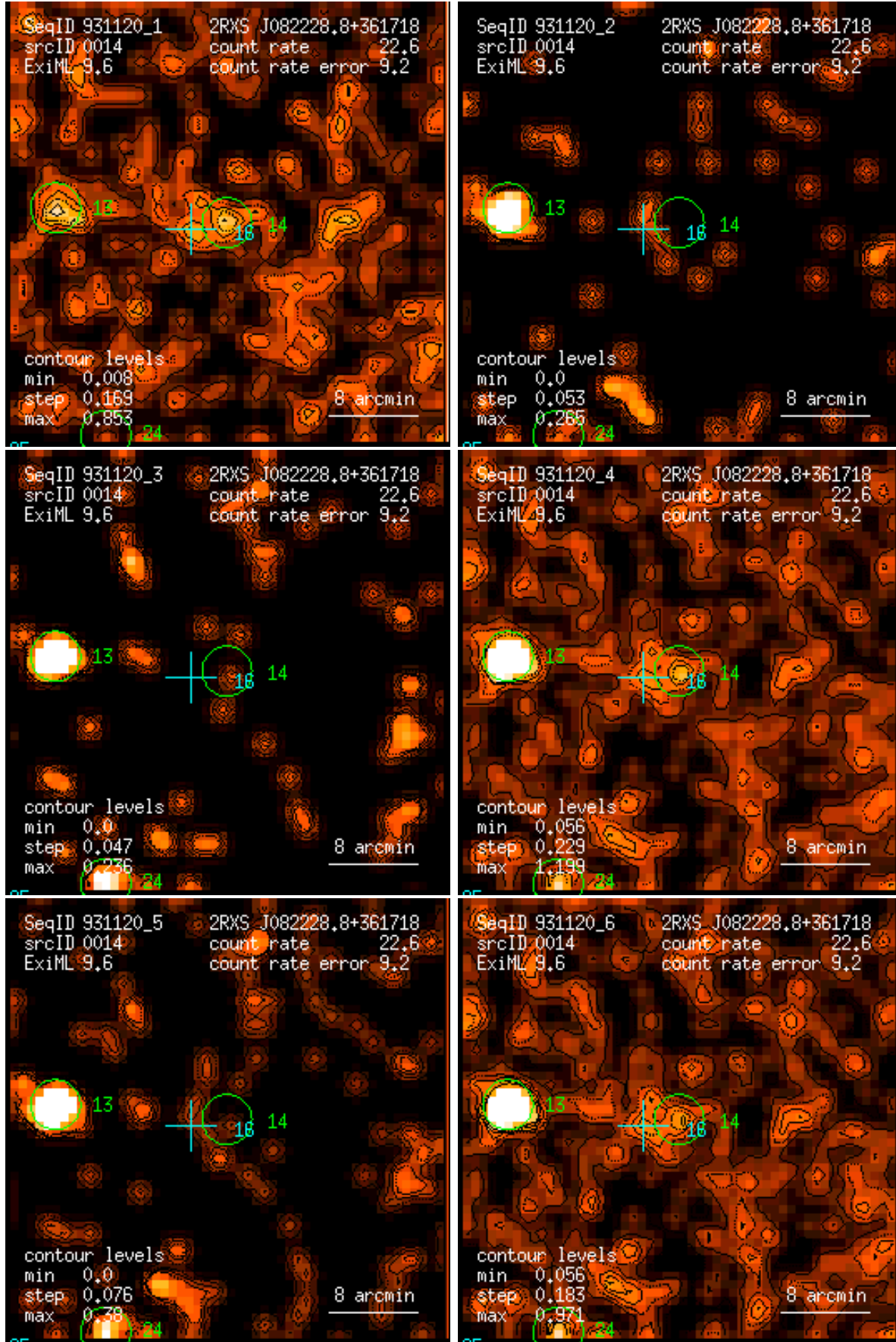
Figure 14: RASS 931120: detection 0014: band rate images, Gaussian filter: (1) PSPC channels 11 – 41, (2) 52 – 90, (3) 91 – 201, (4) 11 – 235, (5) 52 – 201, (6) 11 – 201. Broad band rates in counts/ks. Band rate contour levels in counts/ks/arcmin 2 .
