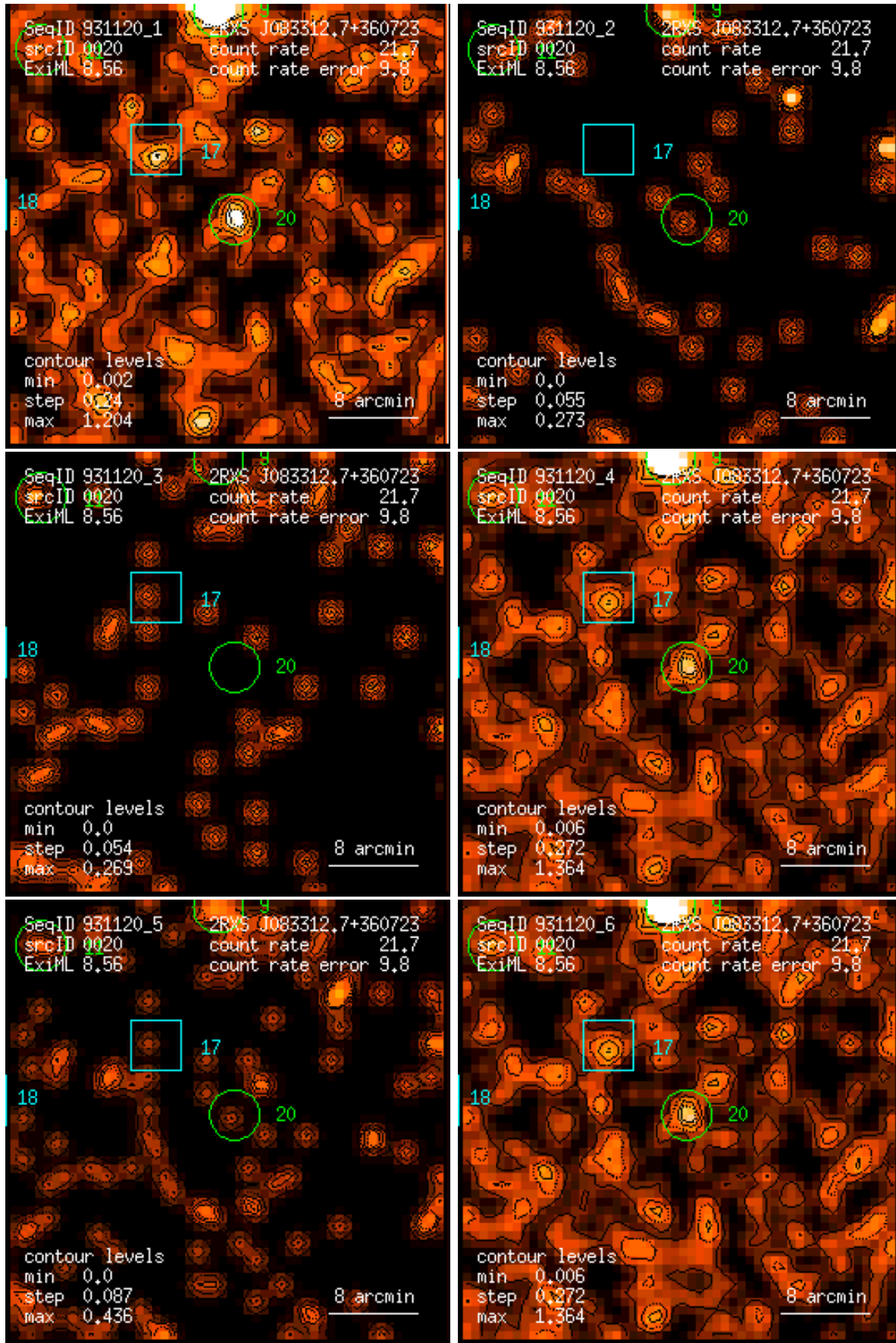
Figure 20: RASS 931120: detection 0020: band rate images, Gaussian filter: (1) PSPC channels 11 – 41, (2) 52 – 90, (3) 91 – 201, (4) 11 – 235, (5) 52 – 201, (6) 11 – 201. Broad band rates in counts/ks. Band rate contour levels in counts/ks/arcmin 2 .
