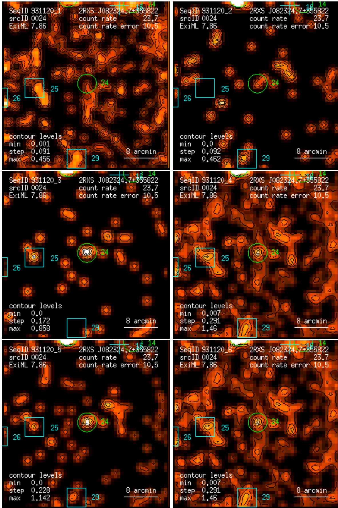
Figure 24: RASS 931120: detection 0024: band rate images, Gaussian filter: (1) PSPC channels 11 – 41, (2) 52 – 90, (3) 91 – 201, (4) 11 – 235, (5) 52 – 201, (6) 11 – 201. Broad band rates in counts/ks. Band rate contour levels in counts/ks/arcmin 2 .
