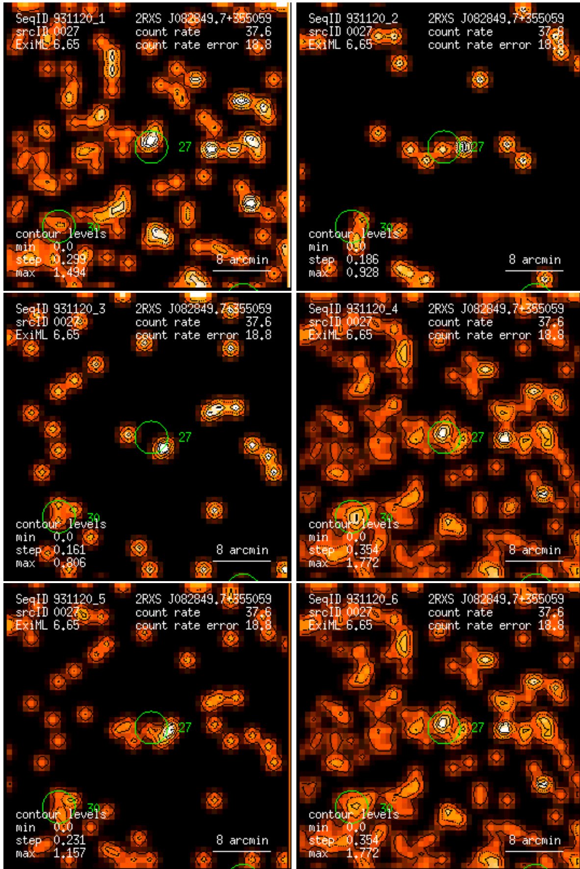
Figure 27: RASS 931120: detection 0027: band rate images, Gaussian filter: (1) PSPC channels 11 – 41, (2) 52 – 90, (3) 91 – 201, (4) 11 – 235, (5) 52 – 201, (6) 11 – 201. Broad band rates in counts/ks. Band rate contour levels in counts/ks/arcmin 2 .
