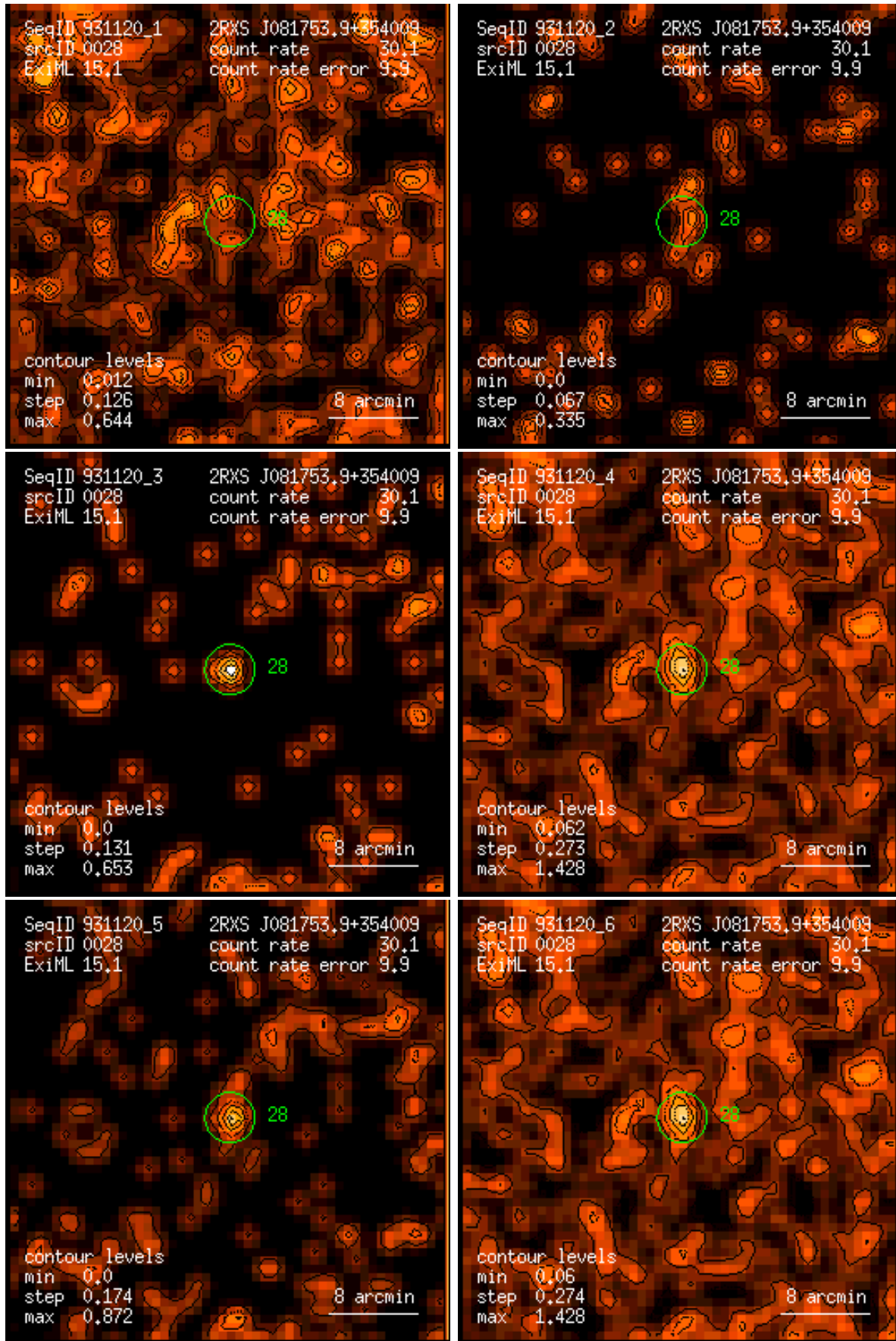
Figure 28: RASS 931120: detection 0028: band rate images, Gaussian filter: (1) PSPC channels 11 – 41, (2) 52 – 90, (3) 91 – 201, (4) 11 – 235, (5) 52 – 201, (6) 11 – 201. Broad band rates in counts/ks. Band rate contour levels in counts/ks/arcmin 2 .
