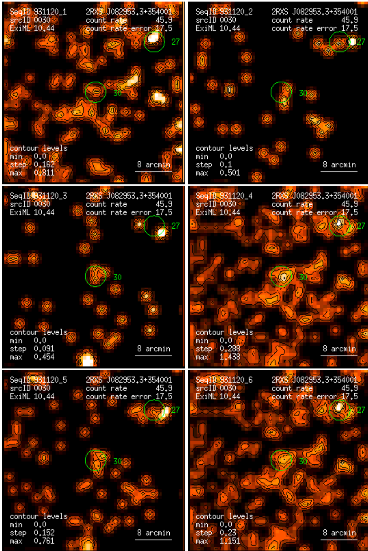
Figure 30: RASS 931120: detection 0030: band rate images, Gaussian filter: (1) PSPC channels 11 – 41, (2) 52 – 90, (3) 91 – 201, (4) 11 – 235, (5) 52 – 201, (6) 11 – 201. Broad band rates in counts/ks. Band rate contour levels in counts/ks/arcmin 2 .
