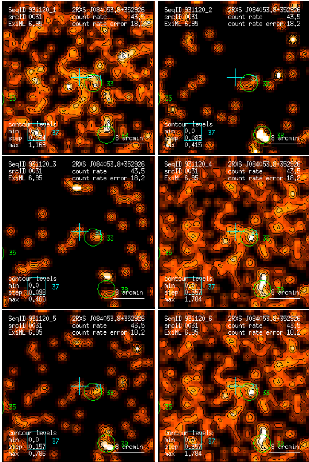
Figure 31: RASS 931120: detection 0031: band rate images, Gaussian filter: (1) PSPC channels 11 – 41, (2) 52 – 90, (3) 91 – 201, (4) 11 – 235, (5) 52 – 201, (6) 11 – 201. Broad band rates in counts/ks. Band rate contour levels in counts/ks/arcmin 2 .
