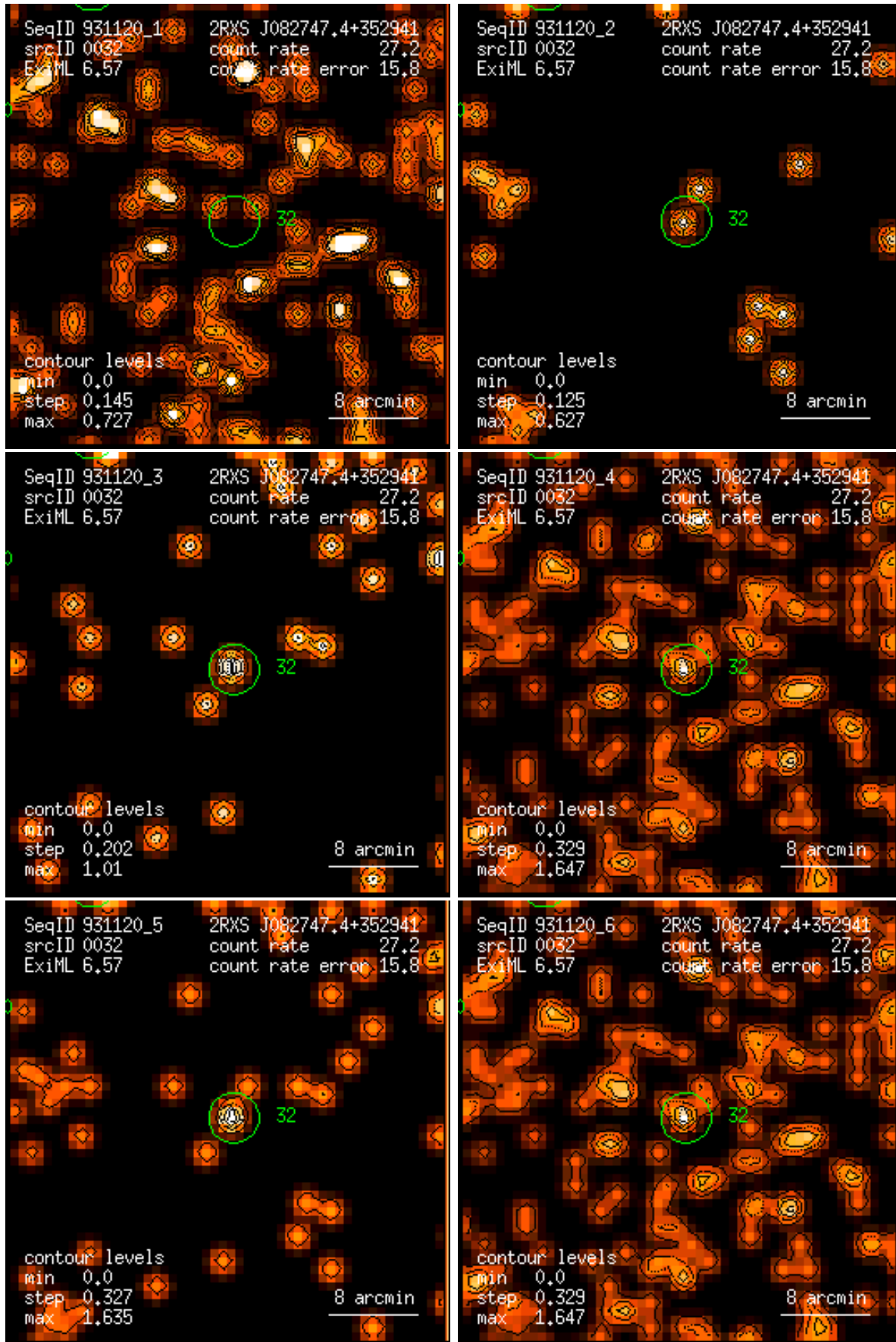
Figure 32: RASS 931120: detection 0032: band rate images, Gaussian filter: (1) PSPC channels 11 – 41, (2) 52 – 90, (3) 91 – 201, (4) 11 – 235, (5) 52 – 201, (6) 11 – 201. Broad band rates in counts/ks. Band rate contour levels in counts/ks/arcmin 2 .
