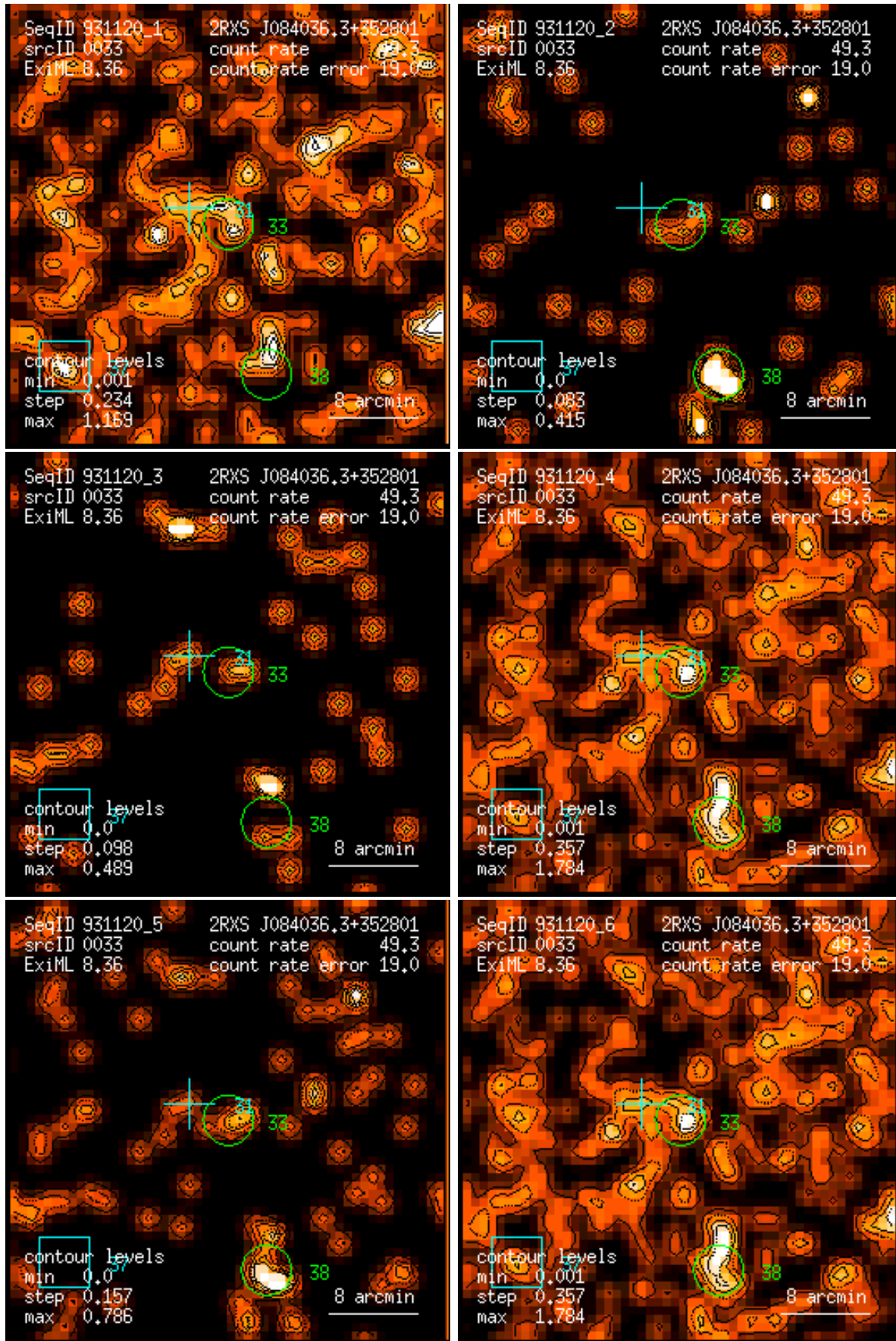
Figure 33: RASS 931120: detection 0033: band rate images, Gaussian filter: (1) PSPC channels 11 – 41, (2) 52 – 90, (3) 91 – 201, (4) 11 – 235, (5) 52 – 201, (6) 11 – 201. Broad band rates in counts/ks. Band rate contour levels in counts/ks/arcmin 2 .
