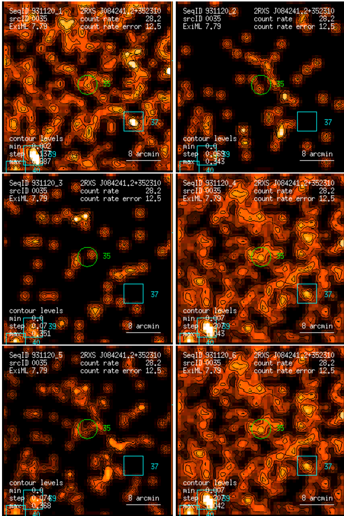
Figure 35: RASS 931120: detection 0035: band rate images, Gaussian filter: (1) PSPC channels 11 – 41, (2) 52 – 90, (3) 91 – 201, (4) 11 – 235, (5) 52 – 201, (6) 11 – 201. Broad band rates in counts/ks. Band rate contour levels in counts/ks/arcmin 2 .
