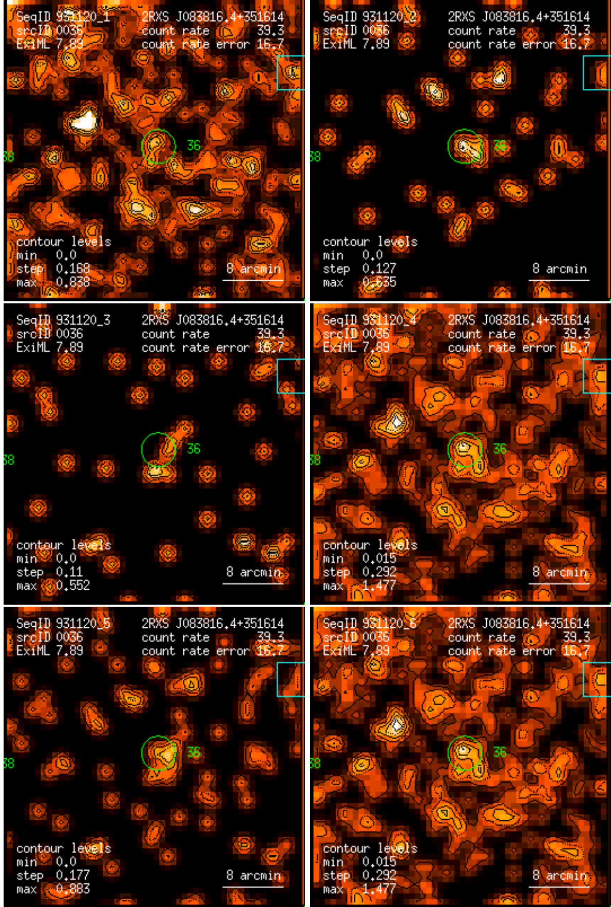
Figure 36: RASS 931120: detection 0036: band rate images, Gaussian filter: (1) PSPC channels 11 – 41, (2) 52 – 90, (3) 91 – 201, (4) 11 – 235, (5) 52 – 201, (6) 11 – 201. Broad band rates in counts/ks. Band rate contour levels in counts/ks/arcmin 2 .
