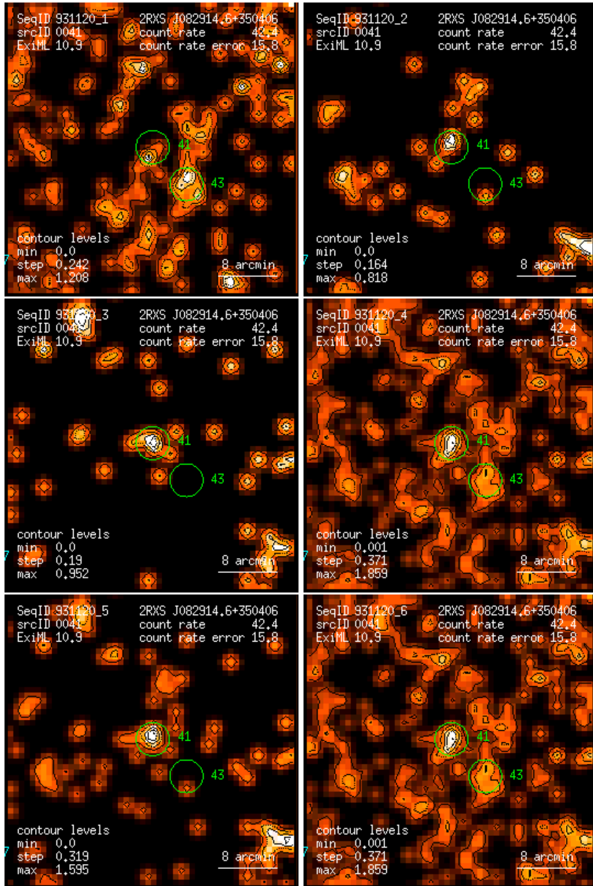
Figure 41: RASS 931120: detection 0041: band rate images, Gaussian filter: (1) PSPC channels 11 – 41, (2) 52 – 90, (3) 91 – 201, (4) 11 – 235, (5) 52 – 201, (6) 11 – 201. Broad band rates in counts/ks. Band rate contour levels in counts/ks/arcmin 2 .
