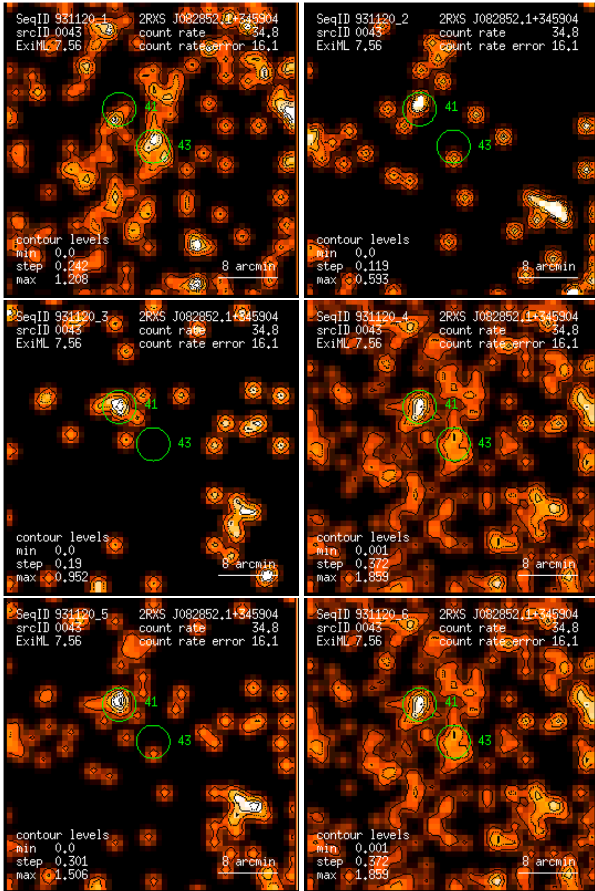
Figure 43: RASS 931120: detection 0043: band rate images, Gaussian filter: (1) PSPC channels 11 – 41, (2) 52 – 90, (3) 91 – 201, (4) 11 – 235, (5) 52 – 201, (6) 11 – 201. Broad band rates in counts/ks. Band rate contour levels in counts/ks/arcmin 2 .
