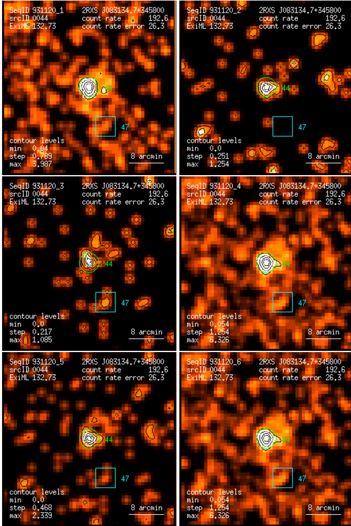
Figure 44: RASS 931120: detection 0044: band rate images, Gaussian filter: (1) PSPC channels 11 – 41, (2) 52 – 90, (3) 91 – 201, (4) 11 – 235, (5) 52 – 201, (6) 11 – 201. Broad band rates in counts/ks. Band rate contour levels in counts/ks/arcmin 2 .
