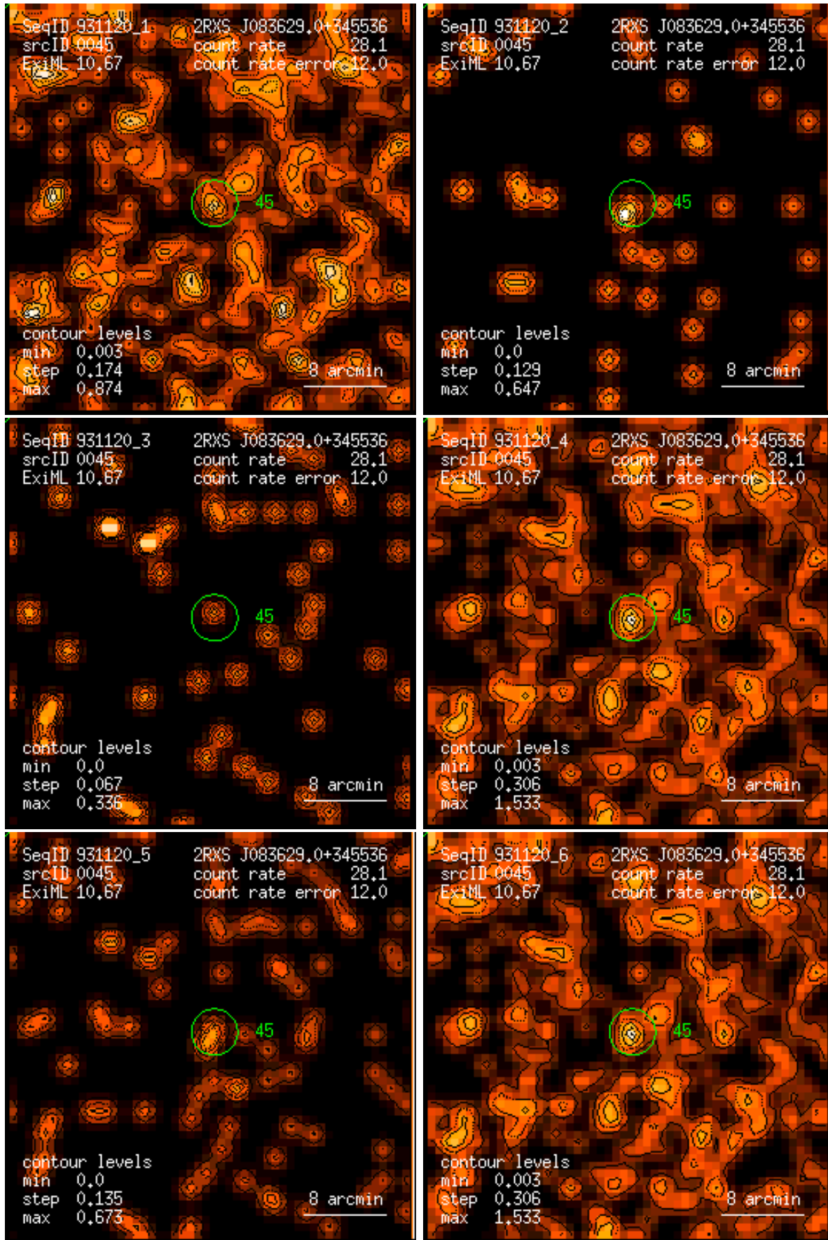
Figure 45: RASS 931120: detection 0045: band rate images, Gaussian filter: (1) PSPC channels 11 – 41, (2) 52 – 90, (3) 91 – 201, (4) 11 – 235, (5) 52 – 201, (6) 11 – 201. Broad band rates in counts/ks. Band rate contour levels in counts/ks/arcmin 2 .
