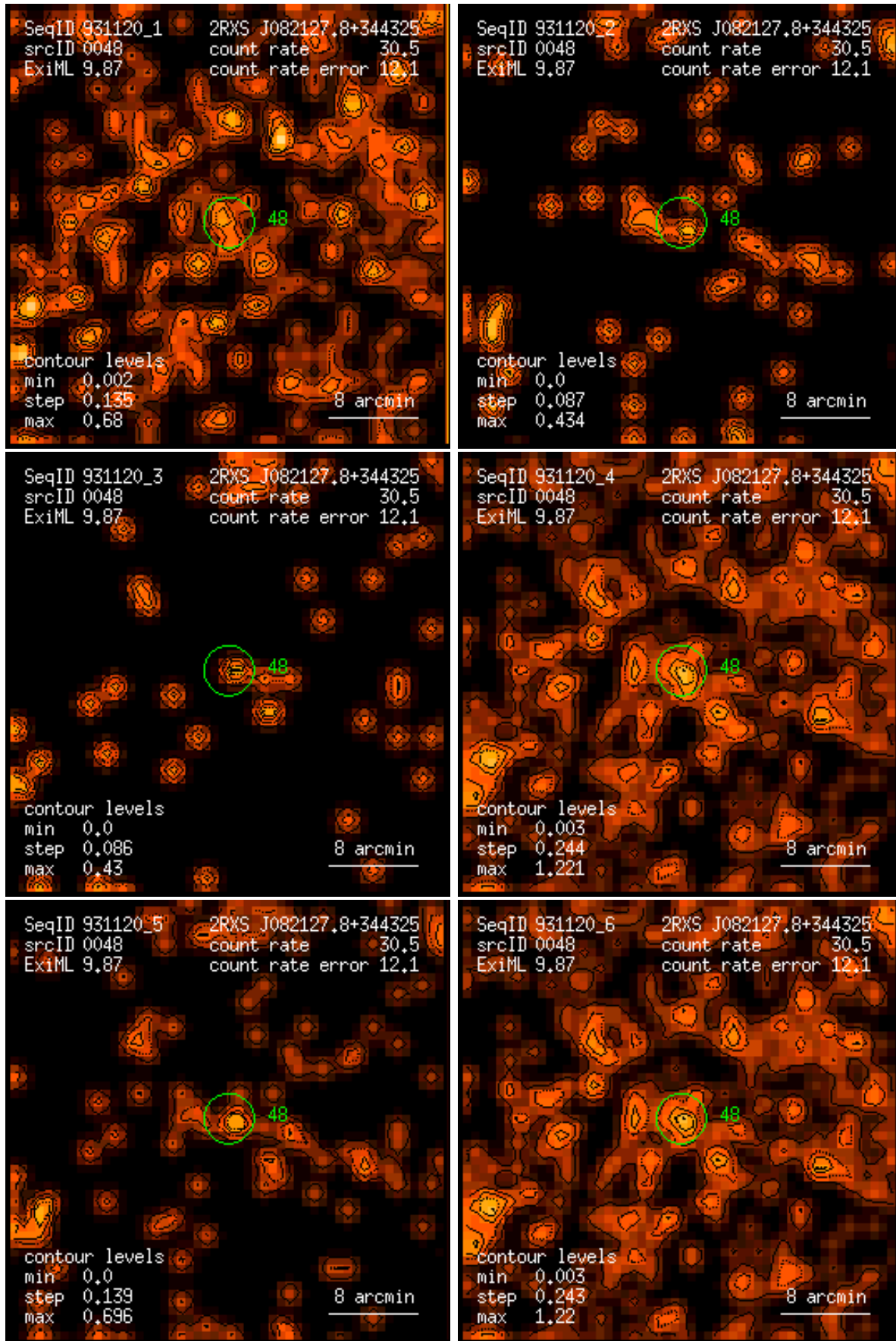
Figure 48: RASS 931120: detection 0048: band rate images, Gaussian filter: (1) PSPC channels 11 – 41, (2) 52 – 90, (3) 91 – 201, (4) 11 – 235, (5) 52 – 201, (6) 11 – 201. Broad band rates in counts/ks. Band rate contour levels in counts/ks/arcmin 2 .
