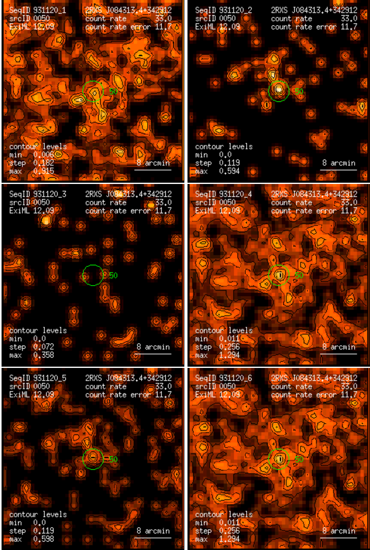
Figure 50: RASS 931120: detection 0050: band rate images, Gaussian filter: (1) PSPC channels 11 – 41, (2) 52 – 90, (3) 91 – 201, (4) 11 – 235, (5) 52 – 201, (6) 11 – 201. Broad band rates in counts/ks. Band rate contour levels in counts/ks/arcmin 2 .
