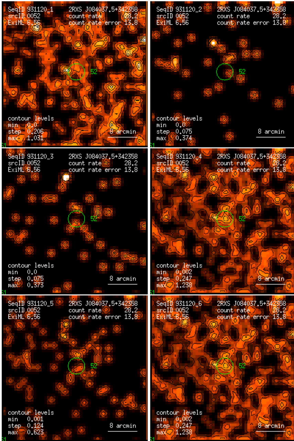
Figure 52: RASS 931120: detection 0052: band rate images, Gaussian filter: (1) PSPC channels 11 – 41, (2) 52 – 90, (3) 91 – 201, (4) 11 – 235, (5) 52 – 201, (6) 11 – 201. Broad band rates in counts/ks. Band rate contour levels in counts/ks/arcmin 2 .
