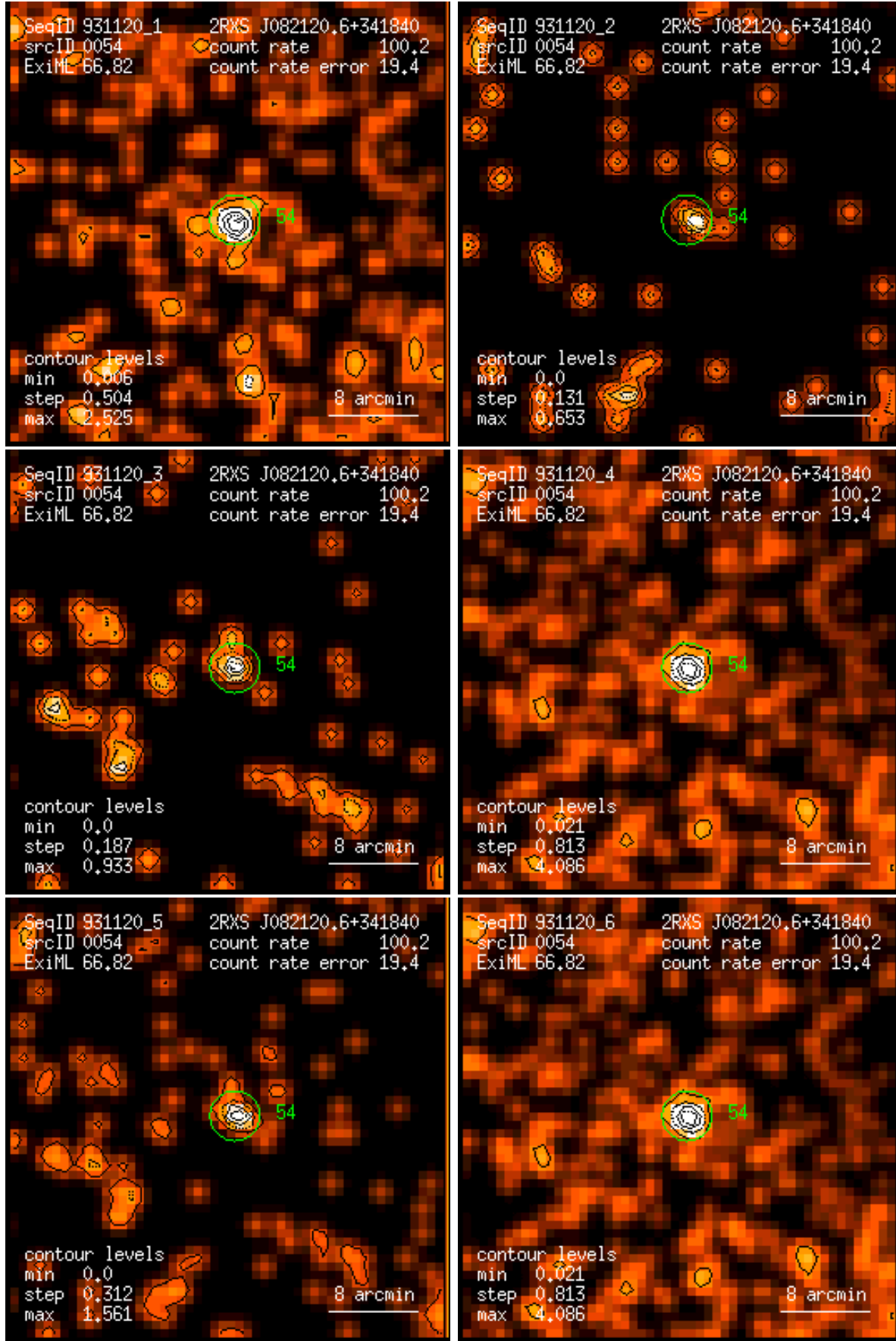
Figure 54: RASS 931120: detection 0054: band rate images, Gaussian filter: (1) PSPC channels 11 – 41, (2) 52 – 90, (3) 91 – 201, (4) 11 – 235, (5) 52 – 201, (6) 11 – 201. Broad band rates in counts/ks. Band rate contour levels in counts/ks/arcmin 2 .
